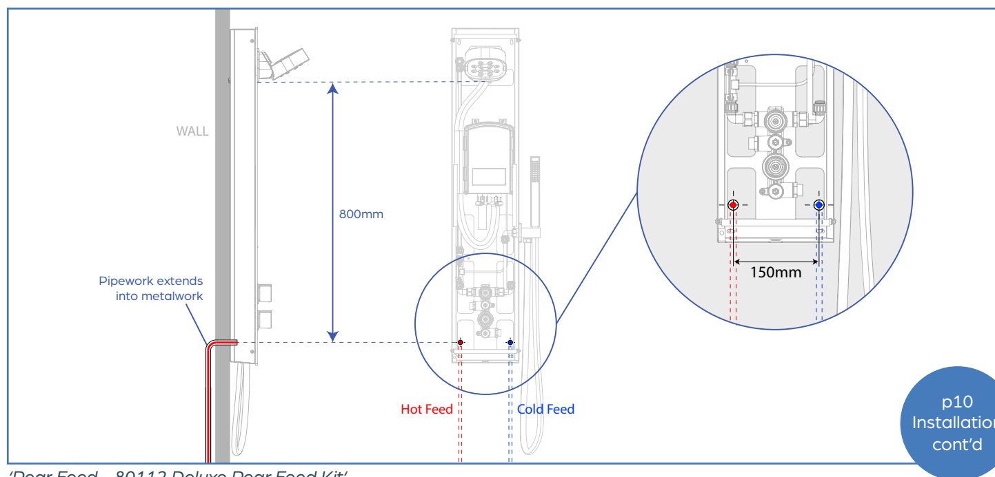
'Rear Feed – 80112 Deluxe Rear Feed Kit'.
