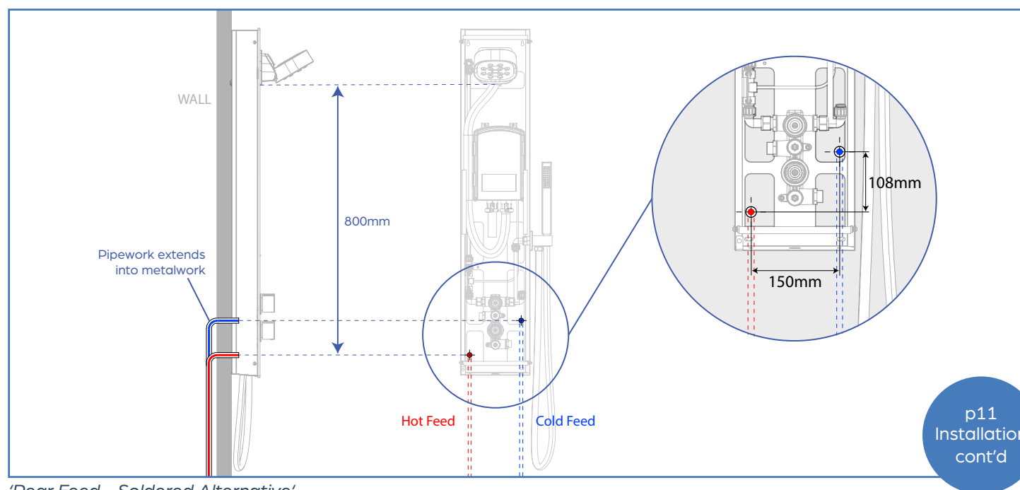
'Rear Feed – Soldered Alternative'.
