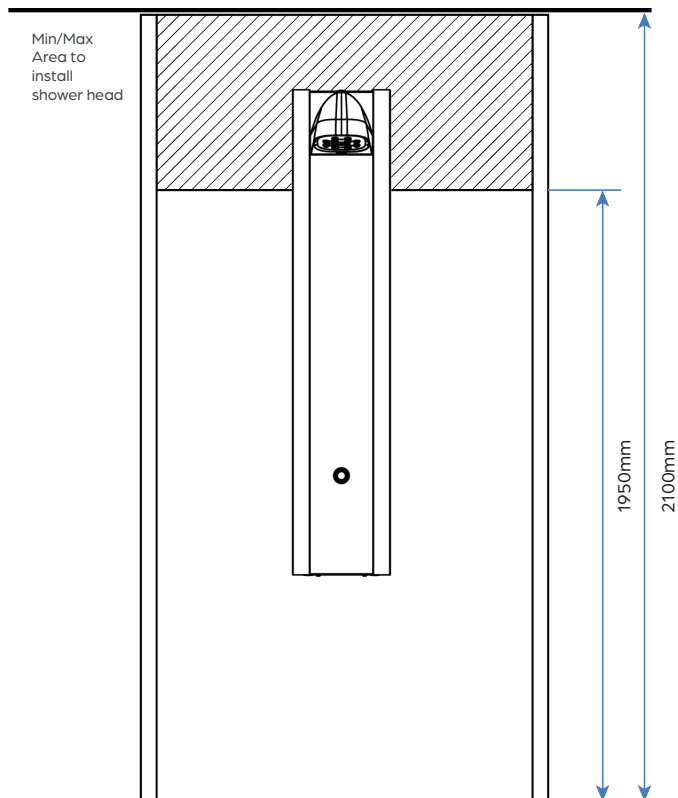
Fixed Head 93011100/93014100
